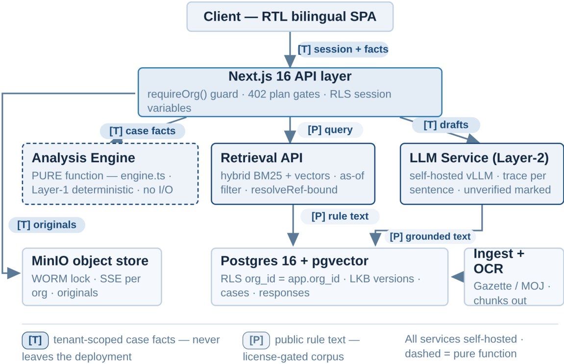
Figure 2-1 — Target architecture with data-sensitivity labels on every flow. All services are self-hosted; case facts (tenant-scoped) never leave the deployment, while rule text (public corpus, license-gated) flows inward only.
