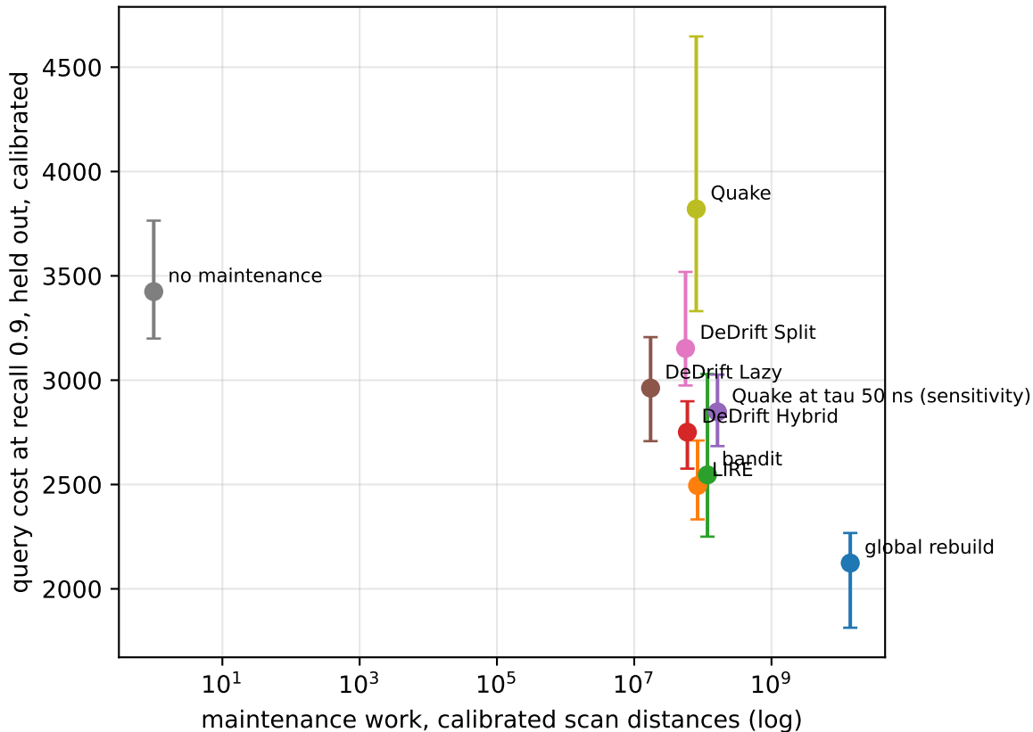
sift1m, mean over 5 seeds, range as bars
