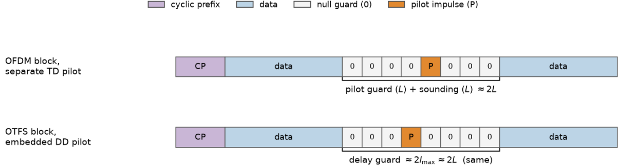
Fig. 1: Pilot overhead in the delay/time domain ( L = l_{\max} + 1 ). A pilot impulse needs a guard of the impulse-response length for its own delay spread and a further such guard to isolate it from data, so an OFDM block with a separate time-domain pilot and an OTFS block with an embedded delay-Doppler pilot both spend about 2L around the pilot. An OTFS block therefore carries the same pilot overhead as the OFDM block.
