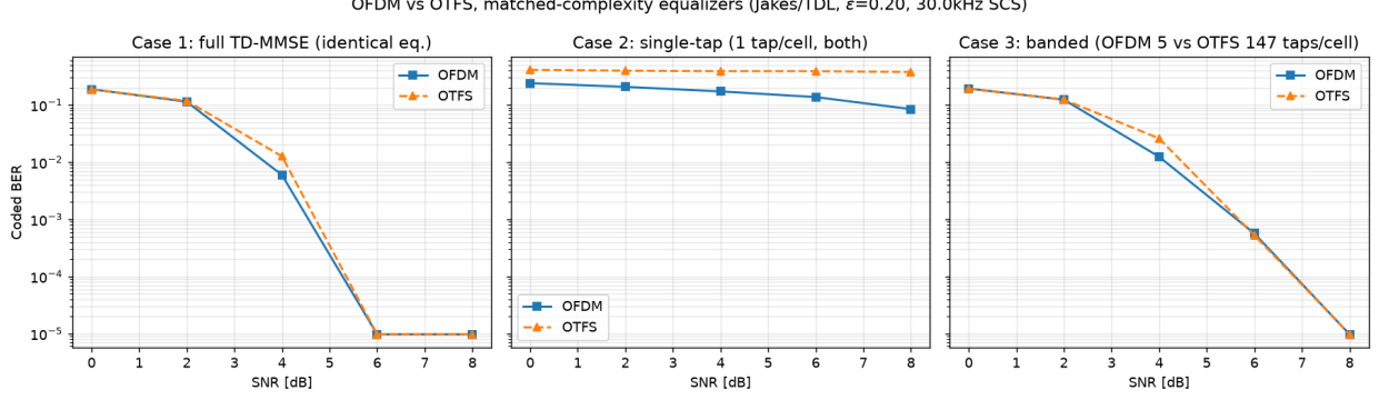
Fig. 2: Matched-complexity OFDM vs. OTFS on a Jakes/TDL channel with fractional delays ( \epsilon=0.2 , 30 kHz SCS, LDPC). Case 1: the same full equalizer makes them equivalent. Case 2: single-tap OFDM far exceeds single-tap OTFS (the FFT diagonalizes delay). Case 3: both floor under finite-band equalization, OTFS lower but with \sim 30\times more taps.
