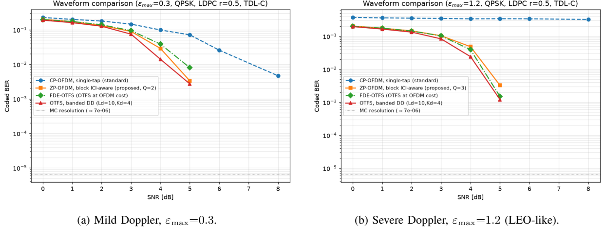
Fig. 3: Coded BER of four receivers on a realistic 3GPP-TDL-C channel (fractional delays, Jakes Doppler, eleven taps), LDPC, M=64 , N=8 . Standard single-tap CP-OFDM lags at mild Doppler and floors above 10^{-1} at severe Doppler. The proposed block ICI-aware ZP-OFDM removes the floor and comes within about 1 dB of the joint banded delay–Doppler OTFS. FDE-OTFS, the OTFS spreading equalized at OFDM complexity, coincides with the proposed ZP-OFDM rather than with joint OTFS, so the spreading gives no gain without the costlier joint equalizer (Remark 2). The dotted line marks the Monte-Carlo resolution.
