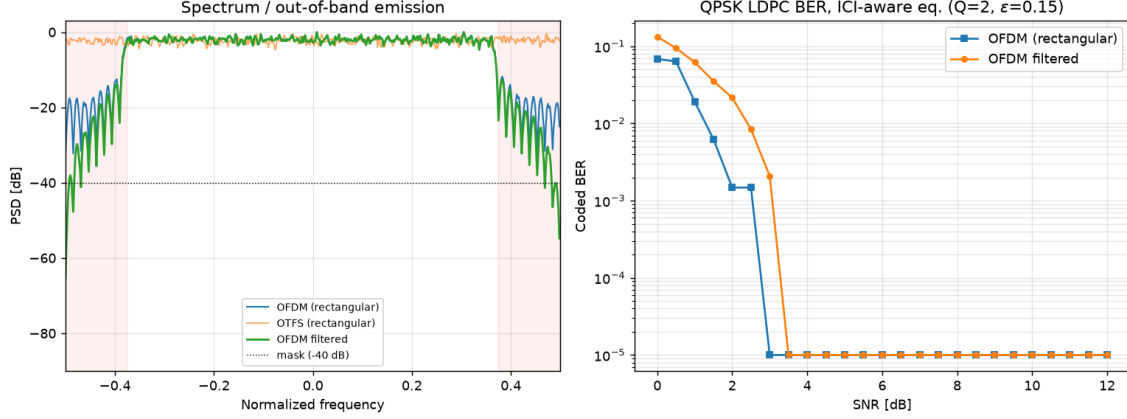
Fig. 4: Pulse shaping. Left: a transmit filter (filtered OFDM) meets a -40 dB spectral mask that rectangular OFDM and rectangular OTFS violate. Right: LDPC-coded QPSK BER with the ICI-aware equalizer. Filtered OFDM tracks the rectangular case within about 1 dB, the edge-subcarrier margin.
