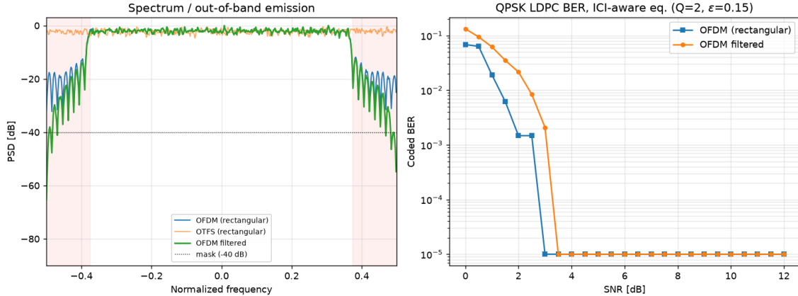
Fig. 3: Pulse shaping. Left: a transmit filter (filtered OFDM) meets a -40 dB spectral mask that rectangular OFDM and rectangular OTFS violate. Right: LDPC-coded QPSK BER with the ICI-aware equalizer. Filtered OFDM tracks the rectangular case within about 1 dB, the edge-subcarrier margin.
