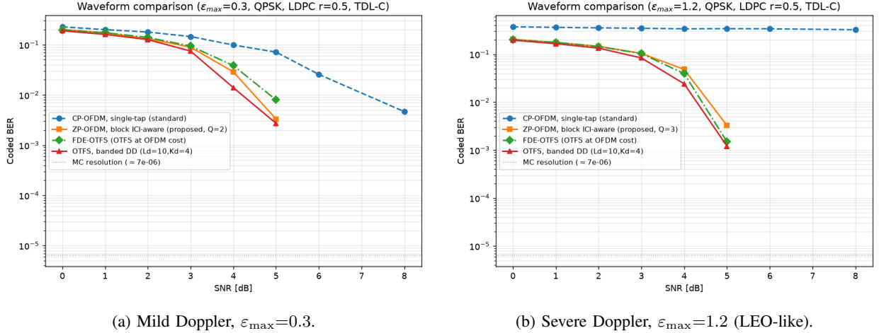
Fig. 2: Coded BER of four receivers on a realistic 3GPP-TDL-C channel (fractional delays, Jakes Doppler, eleven taps), LDPC, M=64 , N=8 . Standard single-tap CP-OFDM lags at mild Doppler and floors above 10^{-1} at severe Doppler. The proposed block ICI-aware ZP-OFDM removes the floor and comes within about 1 dB of the joint banded delay–Doppler OTFS. FDE-OTFS, the OTFS spreading equalized at OFDM complexity, coincides with the proposed ZP-OFDM rather than with joint OTFS, so the spreading gives no gain without the costlier joint equalizer (Remark 2). The dotted line marks the Monte-Carlo resolution.
