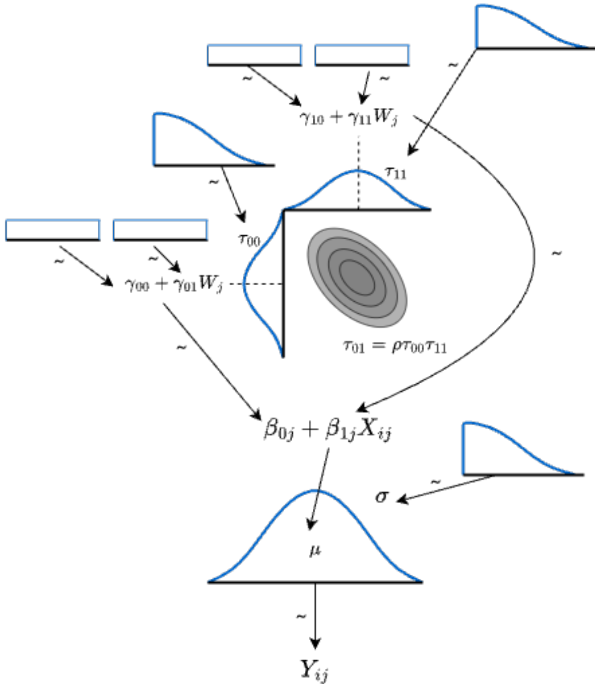
Figure14.1: HLM model diagram
