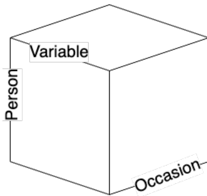
Figure15.1: Cattell's data cube
