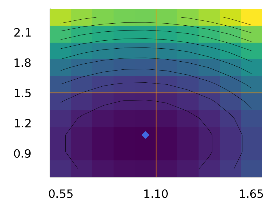
(Param4, Param6)
