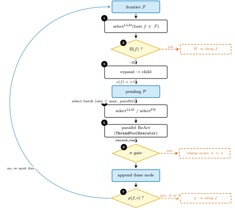
Figure 7: State-machine view of one outer BFTS iteration as a single top-to-bottom flowchart. Steps 1–3 are the inner expansion sub-loop; steps 4–7 are the outer parallel-run loop. Yellow diamonds are the predicate guards ( \Pi, \sigma, \rho ); red dashed boxes on the right are the side-effects each predicate triggers (frontier drop / score clamp / retire). Auxiliary state not drawn here: the per-parent expansion counter e(\cdot) is bumped at step 3 and consulted by \rho at step 7, and the label history H (window W ) is appended at step 5 via record_run and consulted at step 4 to compute the diversity bonus div . Compare with fig. 4, which shows the same loop as a finer-grained control-flow spine with the LLM prompts drawn in.
