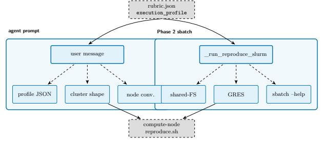
Figure 11: The reproduce_contract.execution_profile field threads from a single rubric artefact into two consumers: the BasicAgent user message (left band, via _format_hpc_appendix ) and the Phase 2 sbatch dispatcher (right band, via _run_reproduce_slurm ). Three runtime probes adapt the dispatched flag set to the local SLURM deployment, so the same rubric dispatches faithfully on heterogeneous clusters without being modified.
