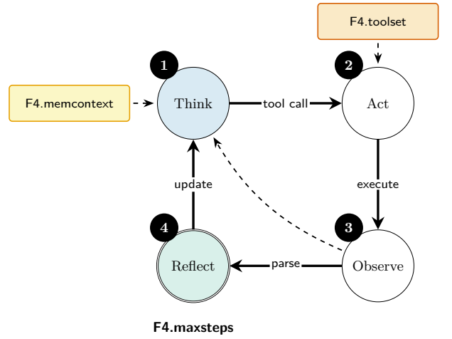
Figure 9: The ReAct loop. Solid edges are the main cycle; the dashed back edge represents an early-exit when the observation already closes the open question.
