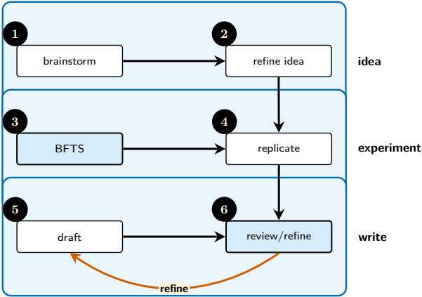
Figure 10: Paper-generation swim lane: idea, experiment, write. Each lane corresponds to a phase; the back edge from review to draft is the only non-monotonic transition (section 4.4).
