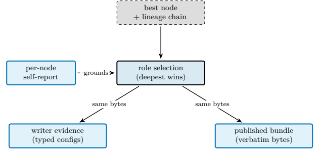
Figure 11: Evidence assembly. The deterministic assembler turns the best node’s lineage into a single selection that feeds two consumers — the writer’s lineage evidence and the published artefact bundle — from the same selected bytes. The per-node self-report (content hashes, success self-assessment, literal build/run commands, captured hardware) grounds the selection, so each contributing file is chosen by recorded metadata; on a path collision the deepest occurrence wins, and a chain deletion removes the file.
