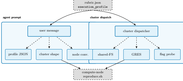
Figure 13: The execution-profile contract threads from a single rubric artefact into two consumers: the replication agent’s prompt (left) and the cluster dispatcher (right). Runtime probes adapt the dispatched resource request to the local scheduler, so one rubric runs faithfully on heterogeneous clusters without being modified.
