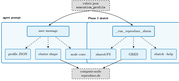
Figure 10: The reproduce_contract.execution_profile field threads from a single rubric artefact into two consumers: the BasicAgent user message (left band, via _format_hpc_appendix ) and the Phase 2 sbatch dispatcher (right band, via _run_reproduce_slurm ). Three runtime probes adapt the dispatched flag set to the local SLURM deployment, so the same rubric dispatches faithfully on heterogeneous clusters without being modified.
