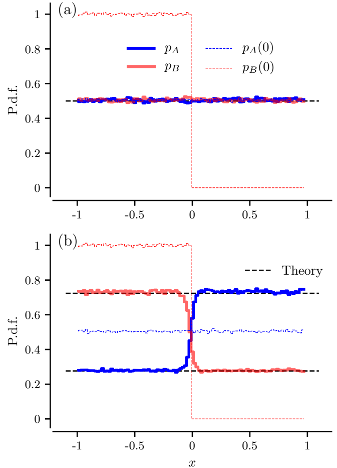
FIG. 1. Demixing of two species in simulations of Langevin equations Eq. (11). Snapshots of the steady-state probability density functions (pdf), p_{A,B}(x, t = 10) , are shown by solid lines for a subcritical value c = 3 < c_{\text{crit}} (a) and a supercritical value c = 5 > c_{\text{crit}} (b). Bin size for pdf estimation \Delta x = 0.02 . Thin lines show corresponding initial densities p_{A,B}(x, t = 0) : homogeneous and inhomogeneous (with an excess on the left) for A and B particles, respectively, and identical in (a) and (b). Theory, Eq. (26), is shown by black dashed lines. Other parameters: number of particles N = 10^6 , integration time step \Delta t = 10^{-5} , s = 1 .
