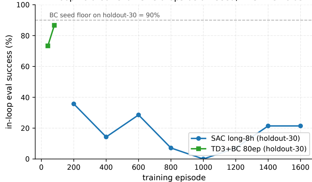
In-loop hold-out eval: SAC drops below seed, TD3+BC holds
