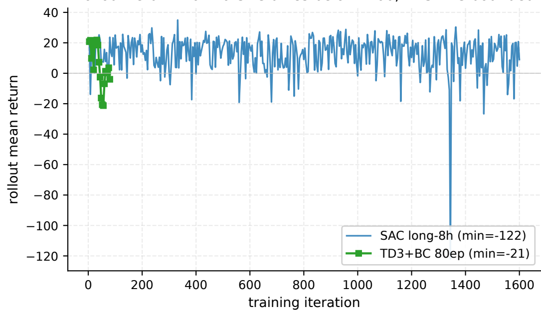
Rollout return: vanilla SAC dives below -100, TD3+BC bounded
