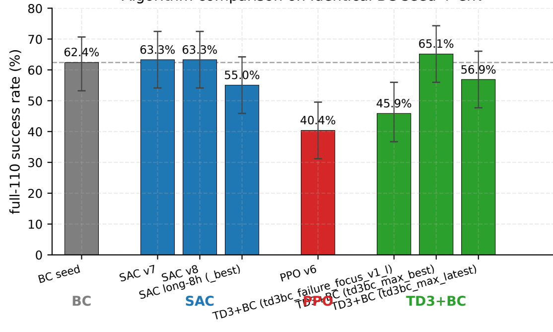
Algorithm comparison on identical BC seed + env
