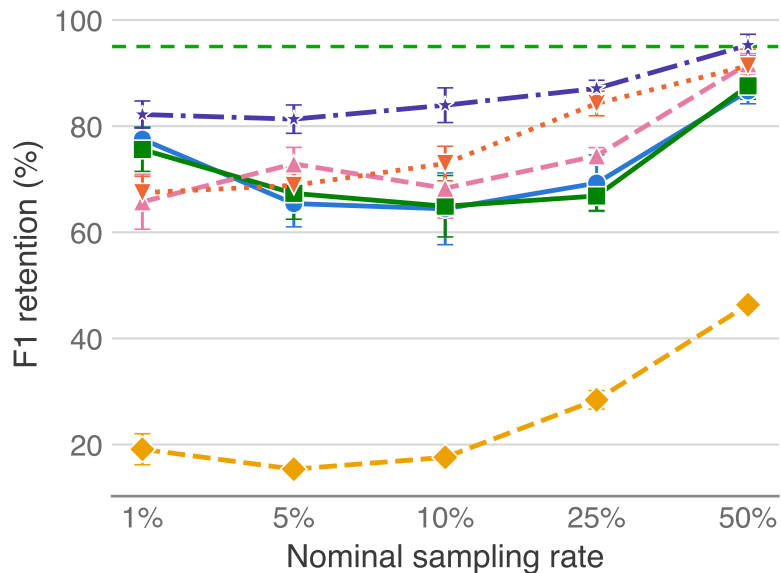
Vessel Classification
