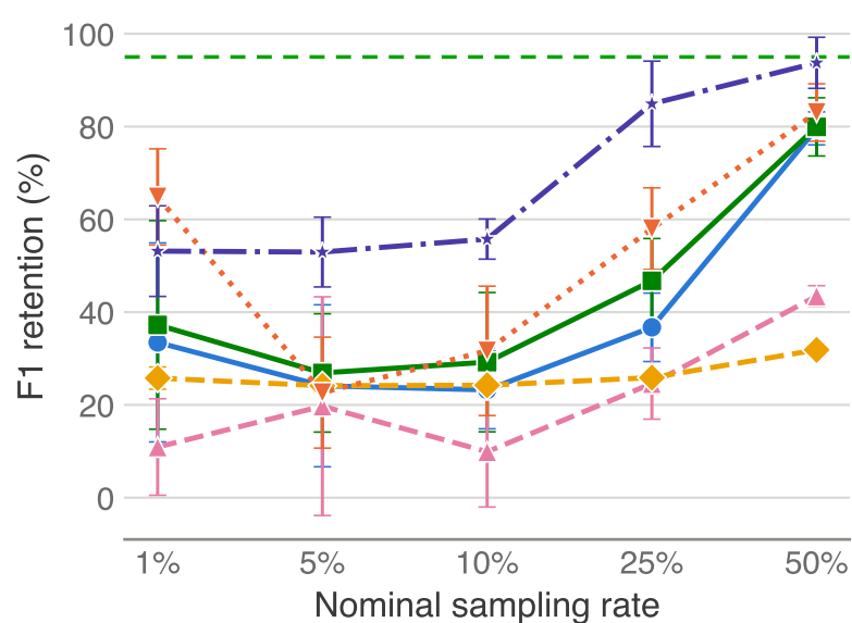
Fishing Detection
