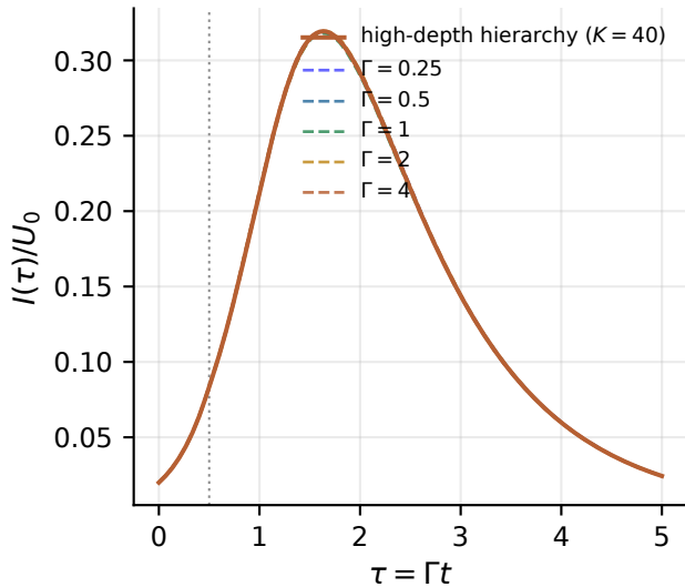
(b) nondimensional collapse
