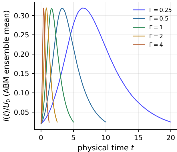
(a) physical-time trajectories
