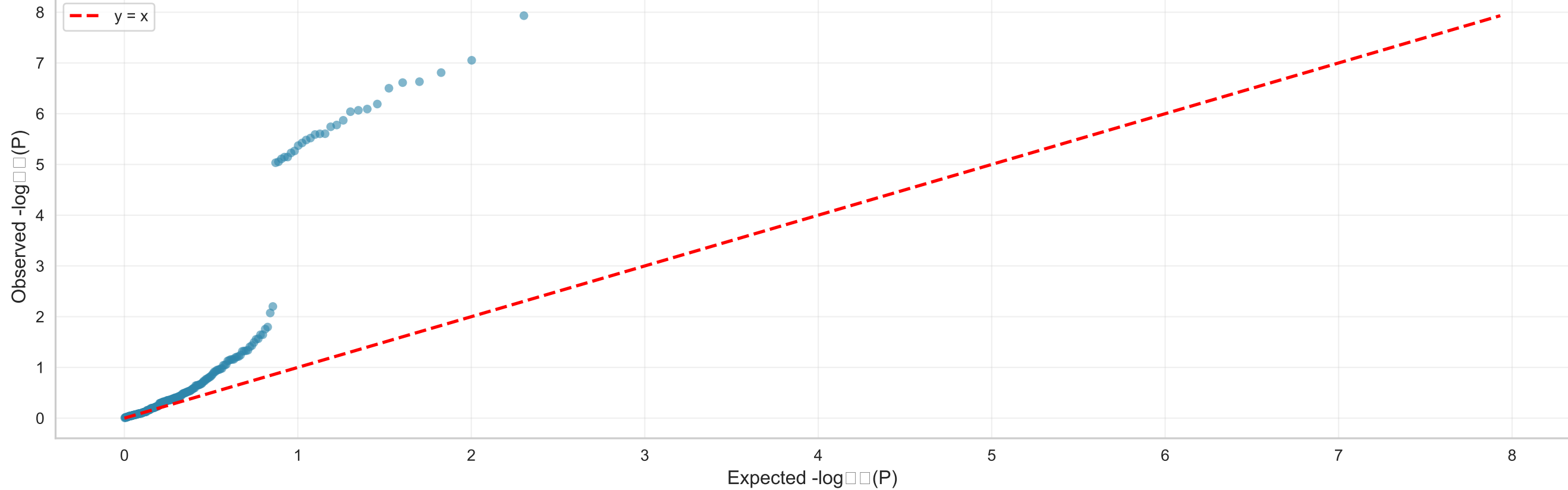
QQ Plot ( \lambda_{GC} = 1.602 ) - Corrected Data
