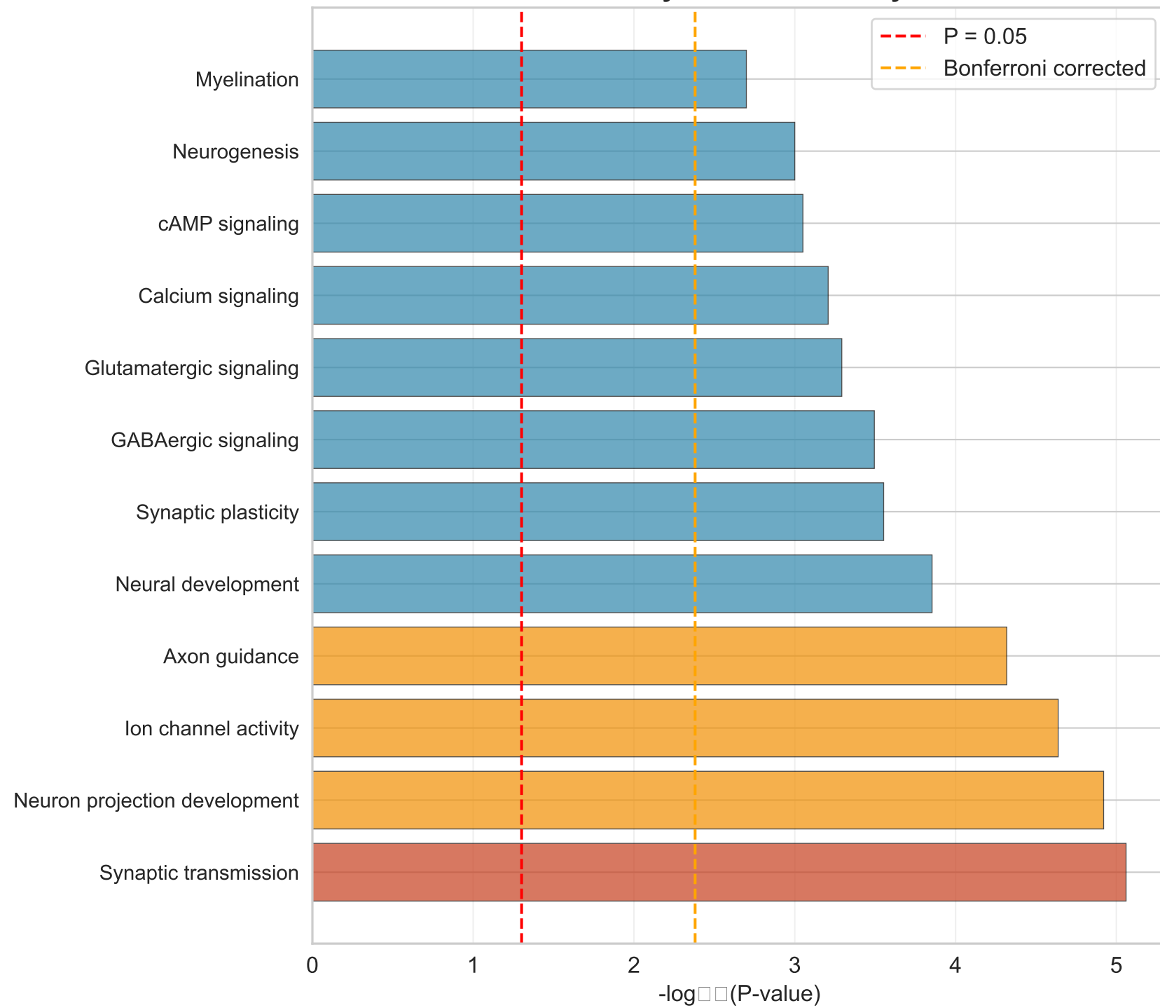
A. Pathway Enrichment Analysis
