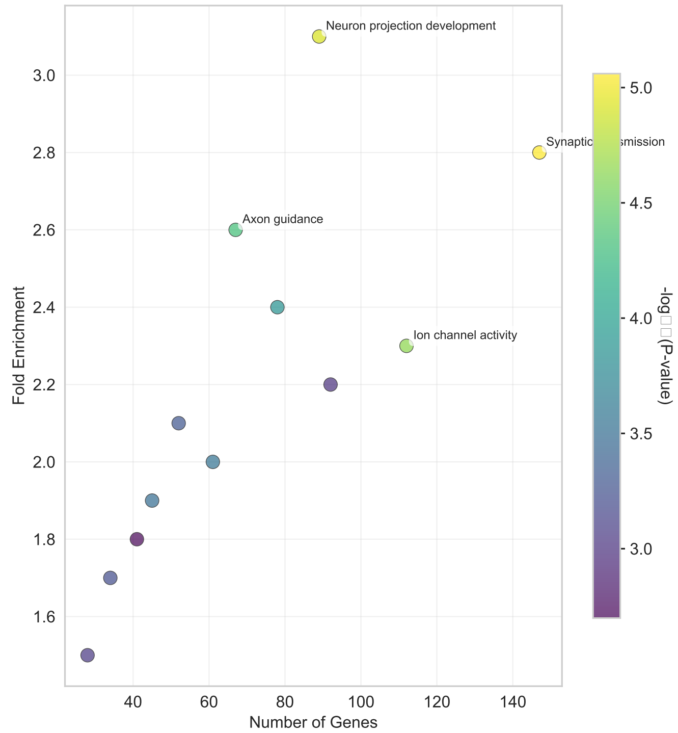
B. Enrichment vs Gene Set Size
