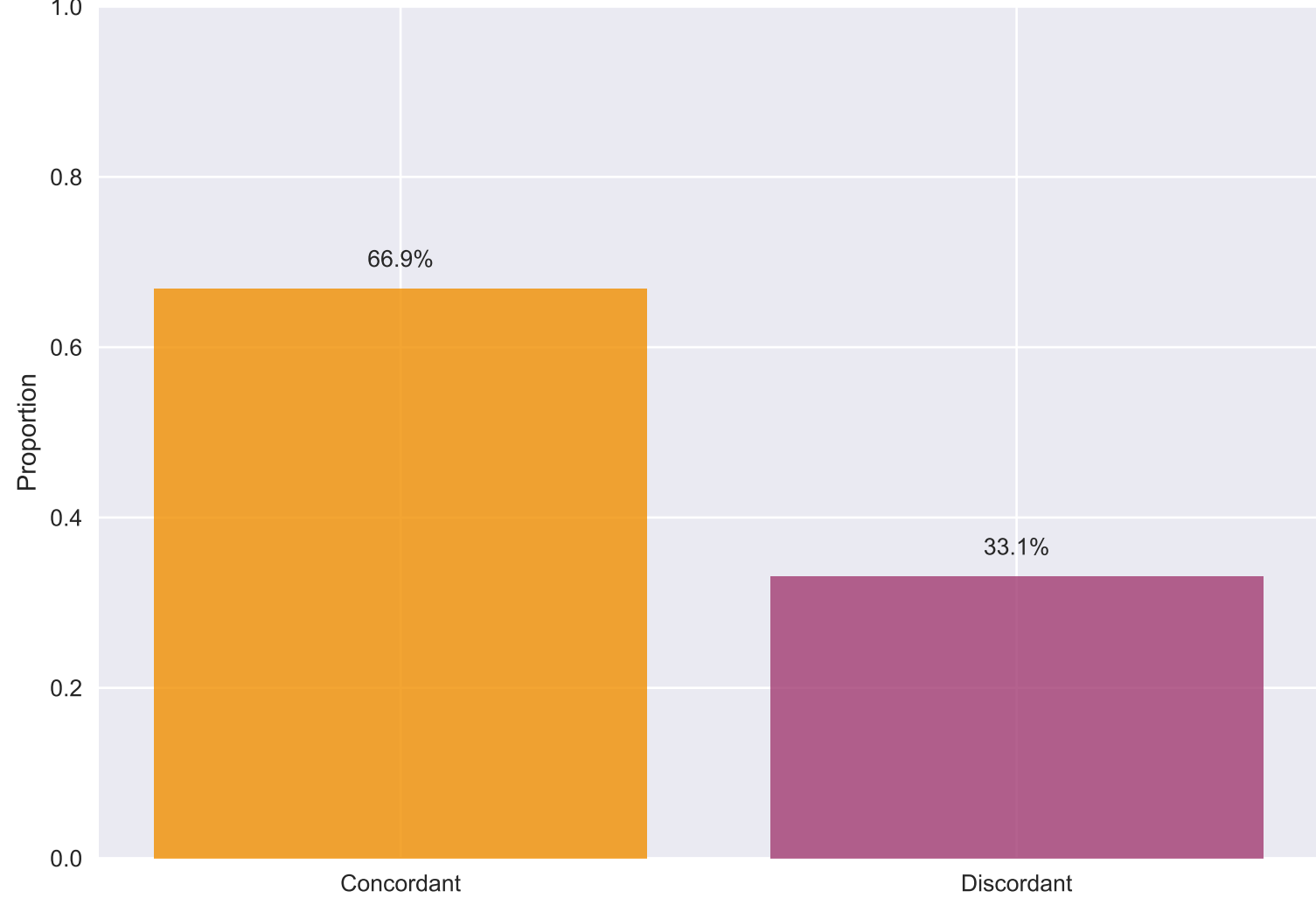
Effect Direction Concordance (66.9%)
