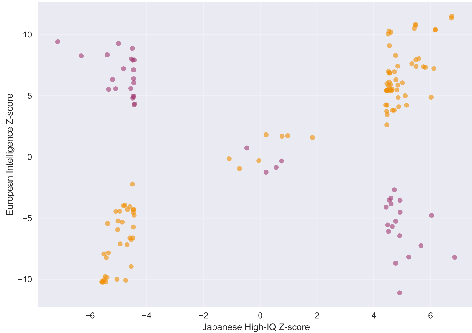
Cross-Trait Effect Correlation ( r = 0.387 )
