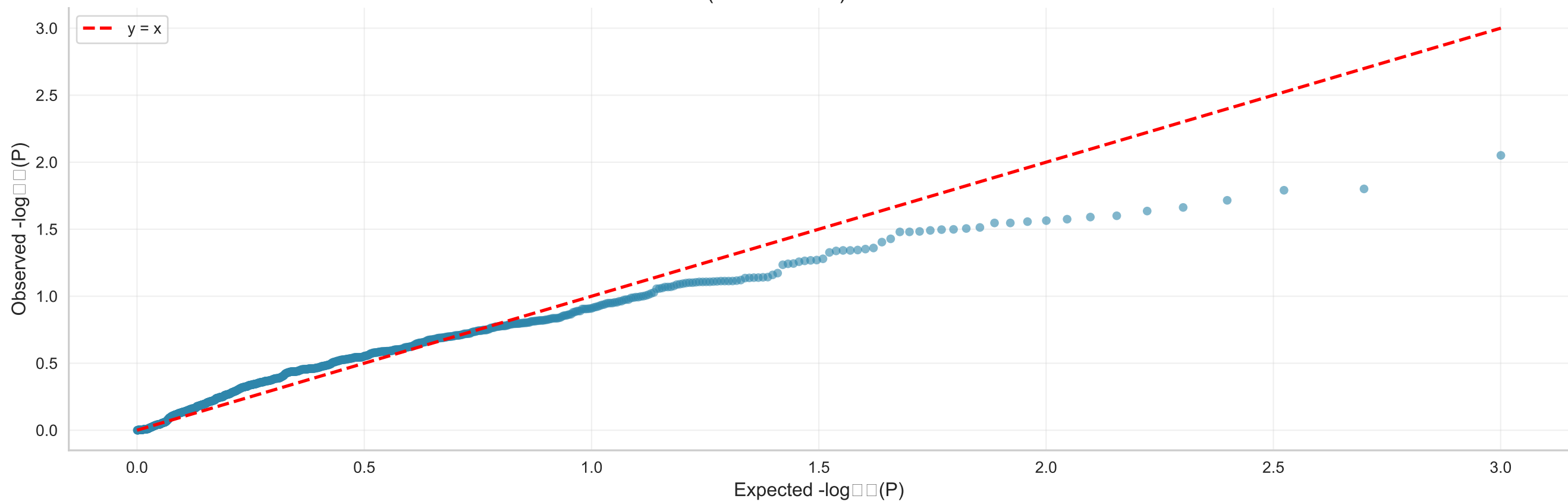
QQ Plot ( \lambda_{GC} = 1.461 ) - Corrected Data
