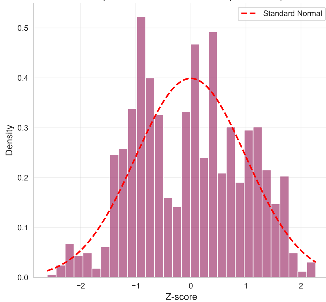
European Z-score Distribution (Corrected)
