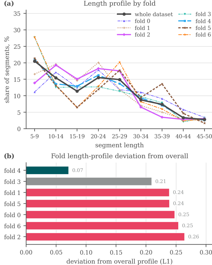
Figure 4: Why the folds of the earlier seven-fold split are not interchangeable: (a) the segment-length profile of each fold against the profile of the whole dataset, (b) the L_1 distance between the two. Fold 4 tracks the overall distribution closely (0.07) while five of the seven folds sit above 0.23. Balancing was done on cleavage motif and homology, not on segment length, so this axis was left free. The same holds for the five-fold split used in the main text, where the imbalance is taxonomic (Table 2).
