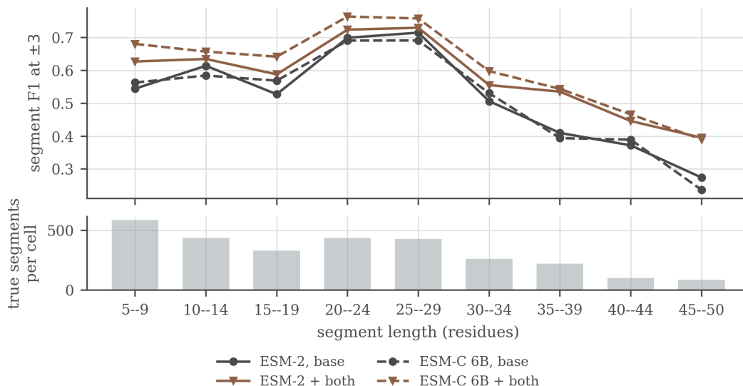
Figure 5: Why a fold’s length profile is not a cosmetic difference. Segment F1 at \pm 3 against the length of the true segment, with the number of true segments in each bin below. Quality is not flat in length: the base architecture scores 0.715 on segments of 25–29 residues and 0.274 on those of 45–50, a spread of 0.441, which is several times any effect this paper measures. A fold holding more long segments is therefore harder before any model touches it, and the folds do differ in length composition (Figure 6). This is what makes them non-exchangeable in the sense Section 6 means. The two additions help most where the base is already strongest and least at the long end, so they do not flatten the curve.
