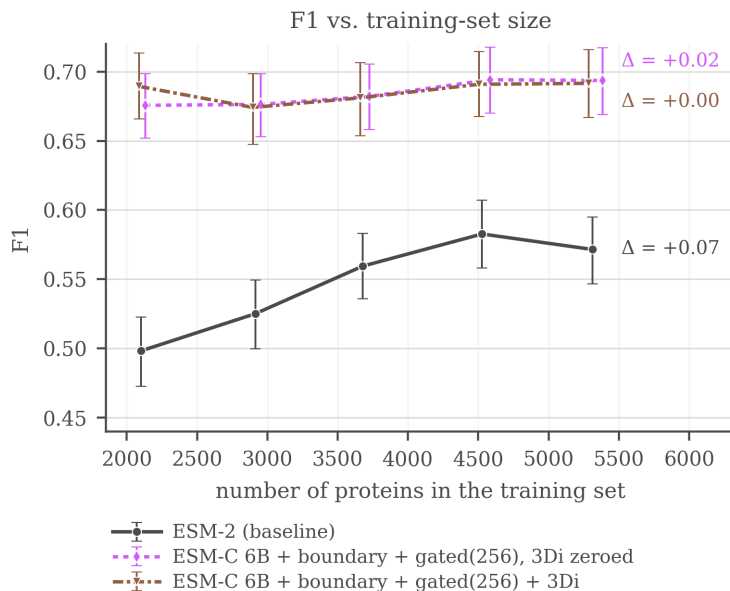
Figure 8: F1 ( \pm 3 ) against the number of training proteins, single-split protocol. ESM-2 rises from 0.498 at 40% of the training folds to 0.583 at 85%, then falls back to 0.572 at 100%, so it is still gaining over most of the range but not at the last point. The ESM-C 6B curves are flat from the smallest size tested, with movement smaller than the bootstrap interval, so nothing is observed saturating: they simply never climb.
