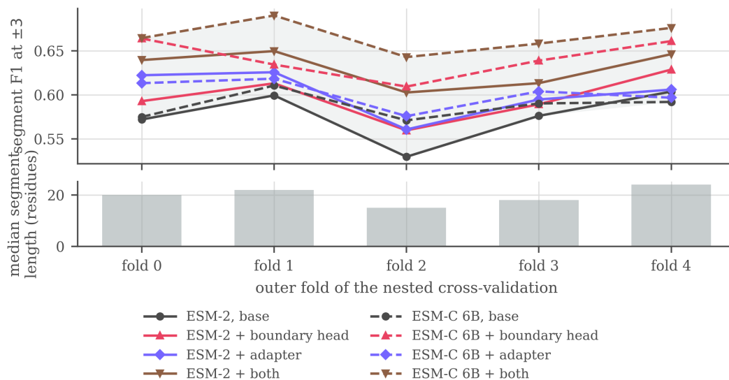
Figure 4: Segment F1 at \pm 3 on each outer fold, every configuration on one axis, with the band between the best and worst configuration shaded, and below it the median length of the true segments each fold contains. The lines move together: fold 2 is the hardest for all eight and fold 1 or 4 the easiest for most, so much of the vertical movement within a line is the fold rather than the architecture. The folds were balanced on homology and cleavage motif, not on segment length, and that free axis tracks the difficulty: ordering them by median segment length and by the base architecture’s score differs in one adjacent swap. Within one configuration the score spans 0.040 to 0.074 across the folds, more than either addition is worth on its own, which is what makes a single split unable to resolve them and pairing by fold necessary. The ordering of configurations is largely preserved from fold to fold, which is why the paired comparisons of Section 5 are stable where the absolute levels are not.
