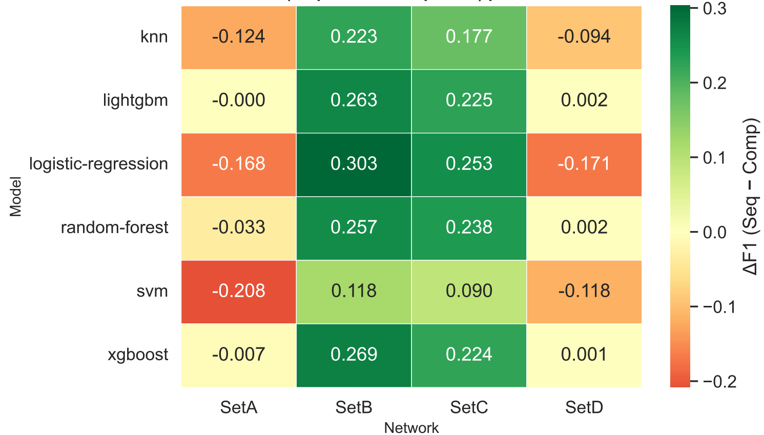
Mean \Delta F1-score (Sequence – Component) per Model and Network
