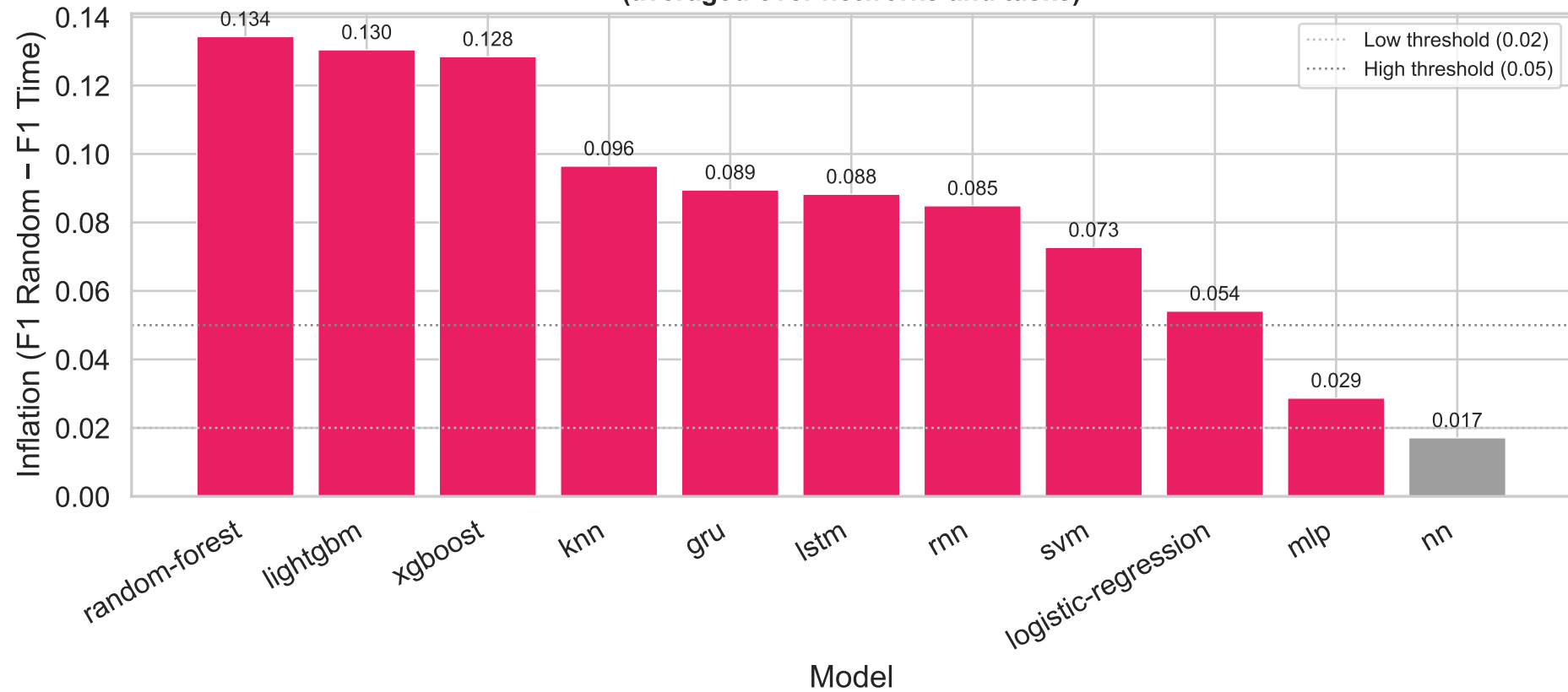
Mean F1 Inflation (Random – Time Split) per Model (averaged over networks and tasks)
