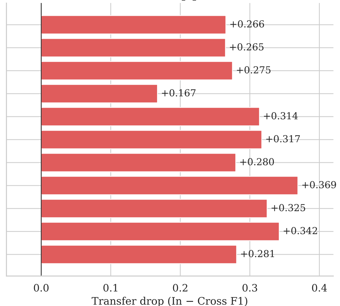
(b) Transfer drop per model
