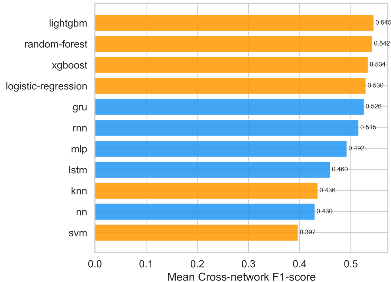
Model Ranking by Cross-network F1 (blue = DL, orange = Classical)
