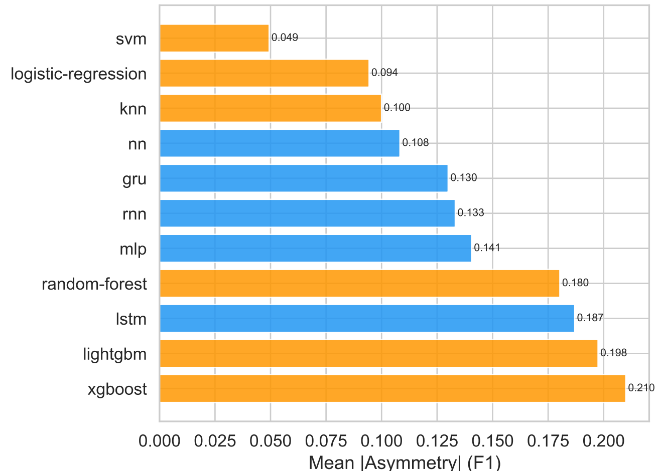
Model Ranking by Transfer Asymmetry (most asymmetric first; blue = DL, orange = Classical)
