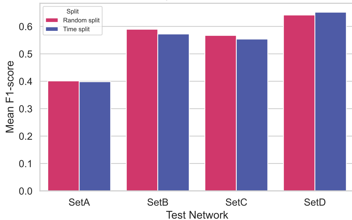
Case Study F1 by Split Strategy per Test Network
