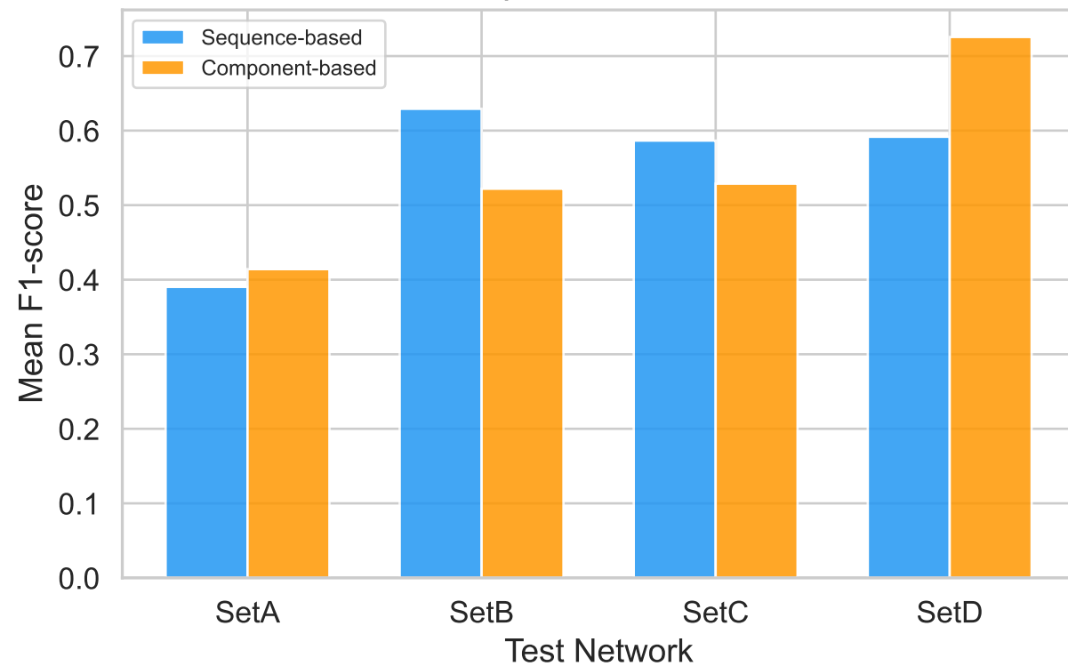
Case Study F1 by Feature Approach per Test Network
