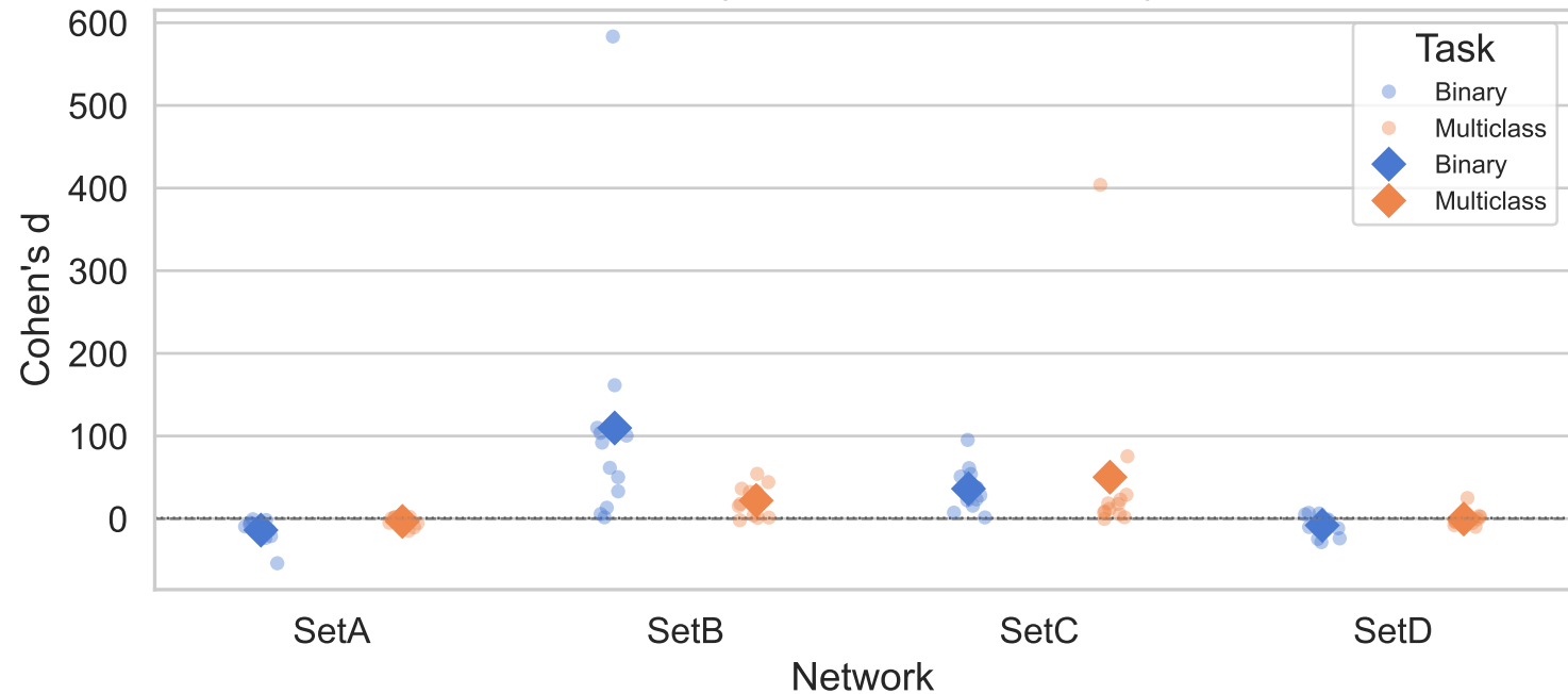
Cohen's d Effect Size (Sequence vs. Component) per Network
