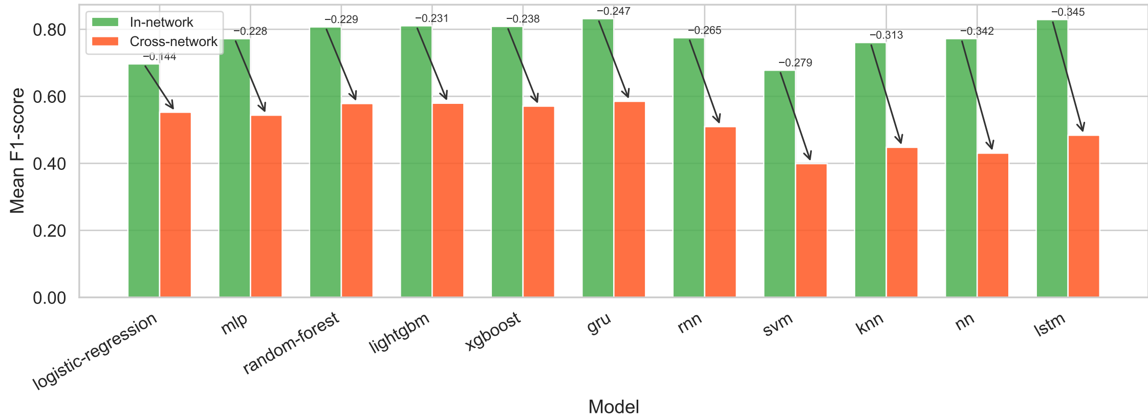
Per-Model Transferability: In-network vs. Cross-network F1 (sorted by transfer drop ascending — most transferable first)
