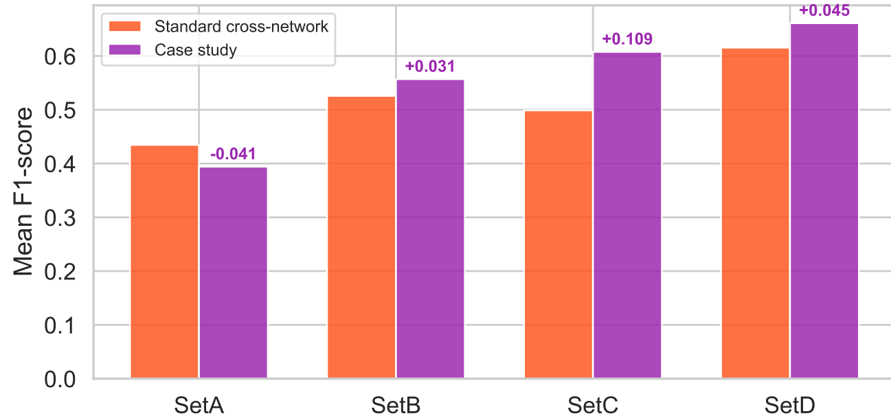
Mean F1 per Test Network Standard Cross-network vs Case Study
