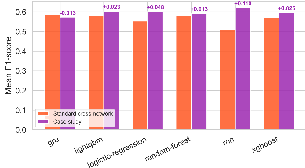
Mean F1 per Model (shared models only) Standard Cross-network vs Case Study
