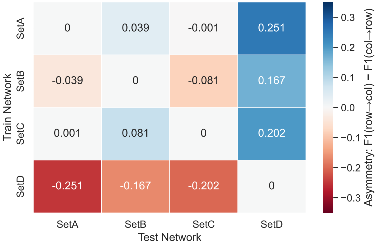
Transfer Asymmetry Matrix (positive = row network is better training source for that column)
