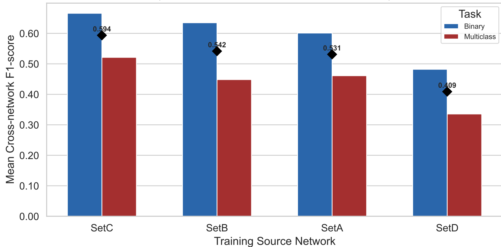
Source Network Quality: Mean Cross-network F1 by Training Source (diamonds = overall mean; sorted best → worst source)
