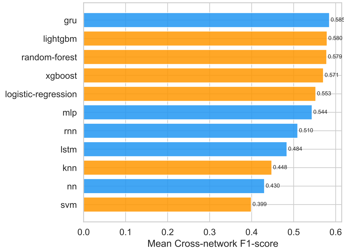
Model Ranking by Cross-network F1 (blue = DL, orange = Classical)
