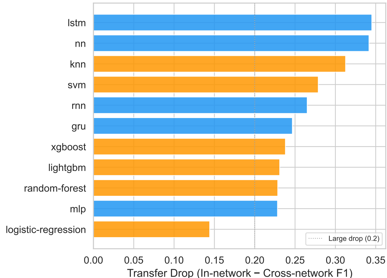
Transfer Drop per Model (blue = DL, orange = Classical)
