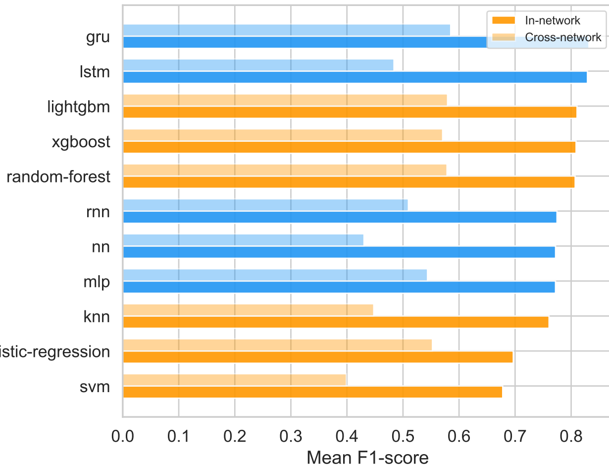
All Models: In-network vs Cross-network F1 (blue = DL, orange = Classical)
