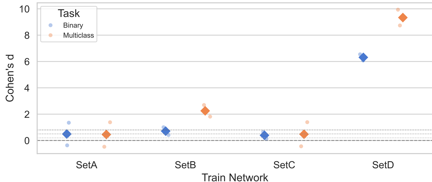
Cohen's d Effect Size: In-network vs. Cross-network (per train network; positive = in-network outperforms cross-network)
