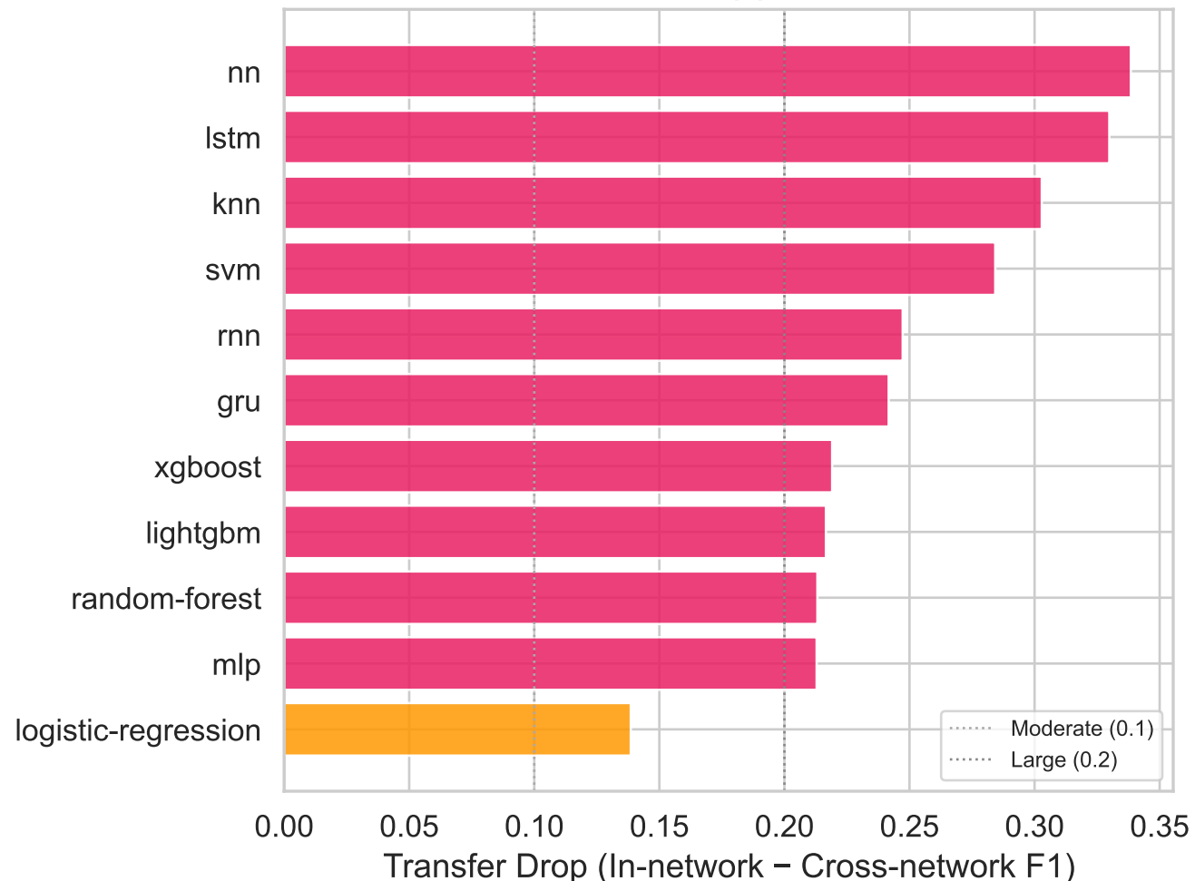
Transfer Drop per Model
