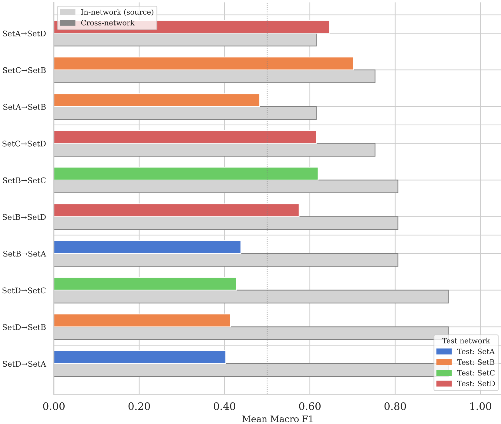
Q3 — In-network vs cross-network F1 for all directed transfers (SetA \leftrightarrow SetC excluded; sorted by cross-network loss, highest first)
