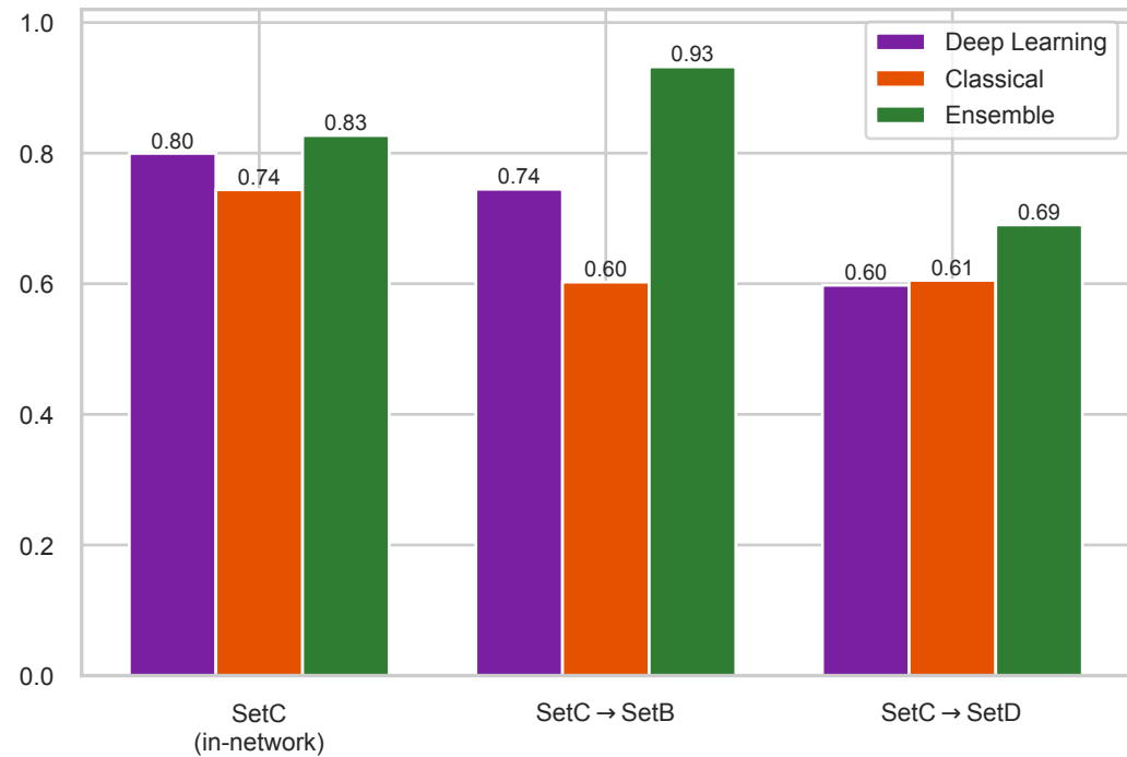
(b) Deployment from SetC (time split)
