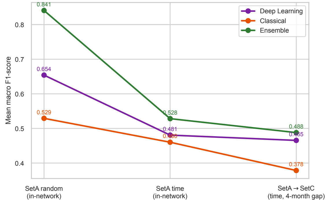
(a) Temporal-generalisation ladder
