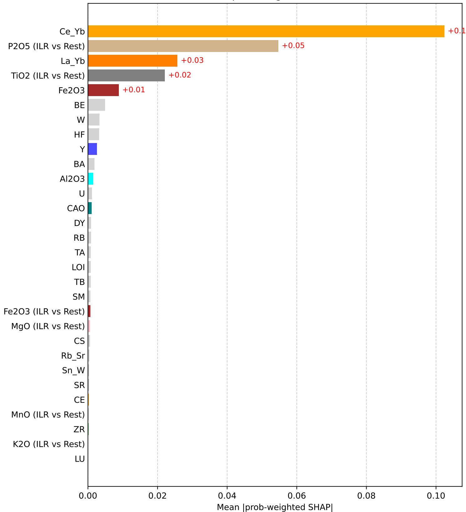
Mean absolute prob-weighted SHAP - moderate
