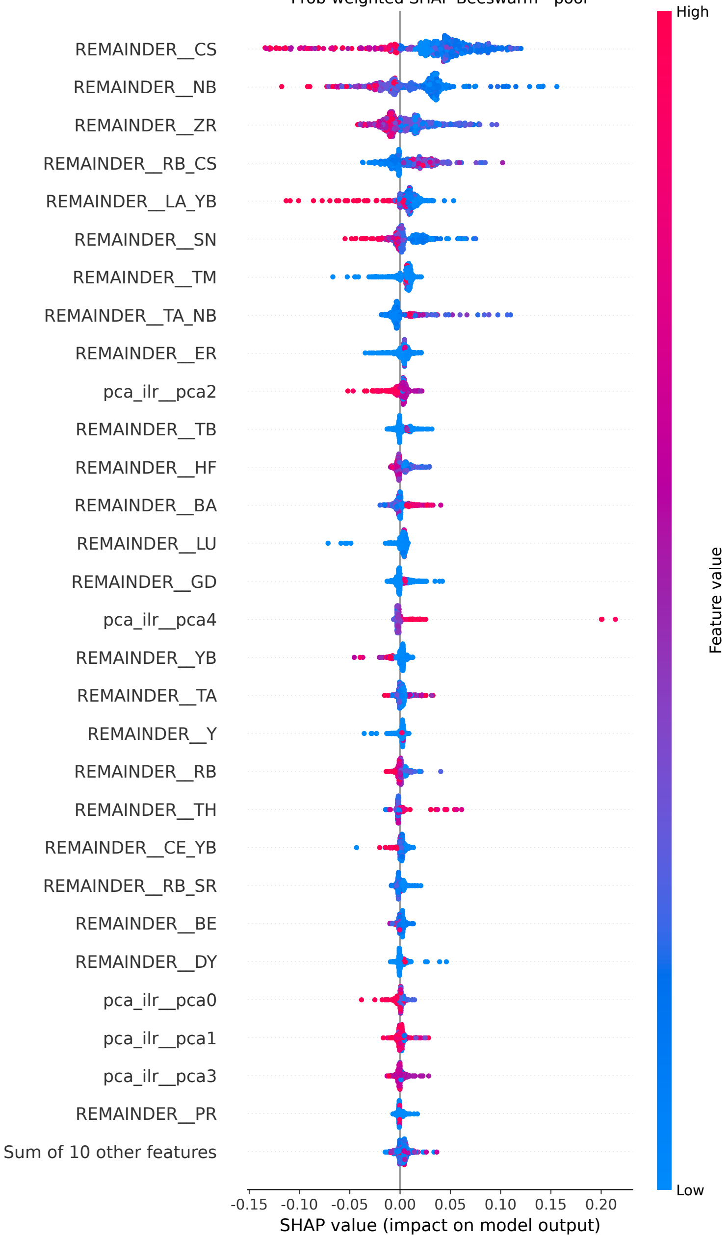
Prob-weighted SHAP Beeswarm - poor
