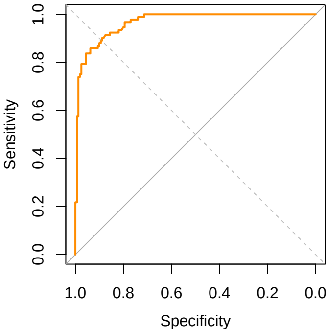
ROC Curve – XGBoost
