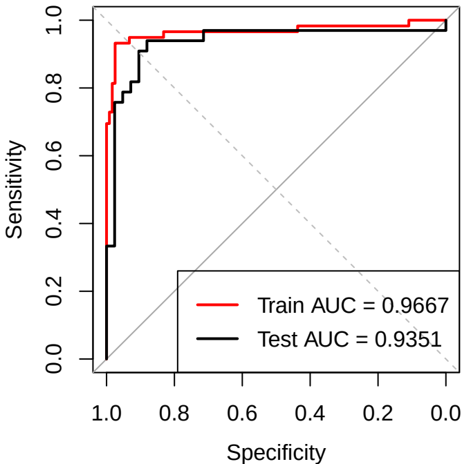
SVM ROC Curve – Train vs Test
