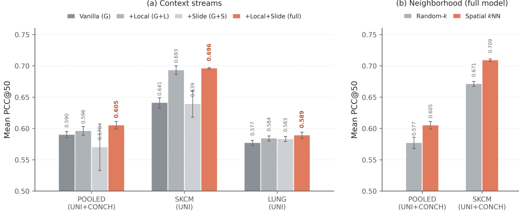
Figure 2: Context-stream ablation: self-attention is the vanilla Transformer backbone; local and slide are the added levers. (a) Backbone (Vanilla, G) plus the local and/or slide pathways, across POOLED (UNI+CONCH) and SKCM/LUNG intra-cohort (UNI). (b) Full model with spatial k NN vs. random- k neighbors (UNI+CONCH); spatially defined neighborhoods are significantly better. Bars are mean \pm std over three seeds.
