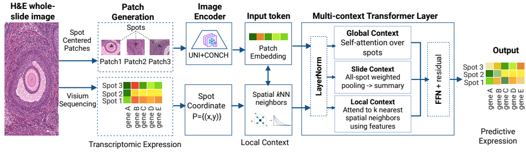
Figure 1: MIST overview. (a) Frozen UNI and/or CONCH embeddings represent spot-centered H&E patches, while spot coordinates define spatial k NN neighborhoods. (b) Each Transformer layer augments the self-attention backbone with two pathways: local spatial-neighbor attention and an attention-pooled slide summary broadcast to all spots. The final spot representations are mapped to predicted gene expression.
