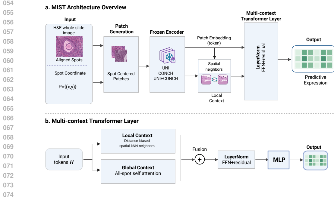
Figure 1: MIST overview. (a) Frozen UNI, CONCH, or combined features turn H&E spot patches into tokens, while coordinate-based k NN edges provide local context. (b) Each layer combines distance-biased local attention with global self-attention before the expression head. Pairwise-distance coordinates ensure invariance to translations, rotations, and reflections.
