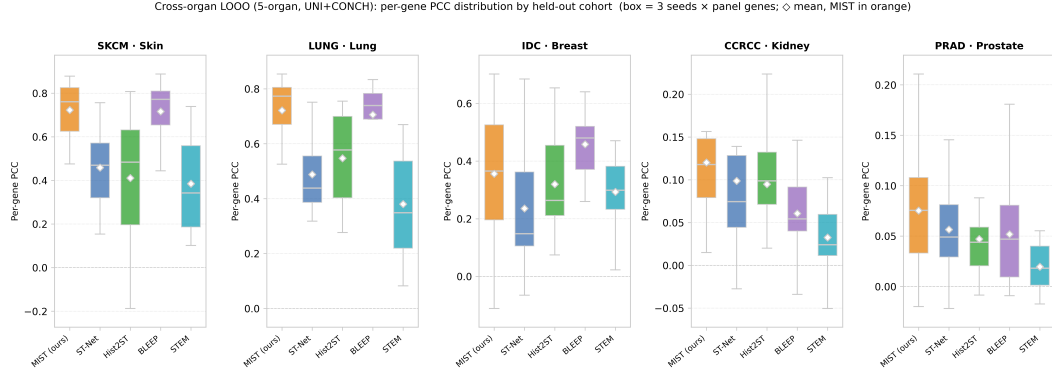
Figure 2: Per-cohort distribution of cross-organ LOOO accuracy (five-organ subset, frozen UNI+CONCH). One panel per held-out cohort; each box is the per-gene PCC pooled over the three seeds and the fold’s leakage-safe panel genes, with the mean marked ( \diamond ). MIST (orange, leftmost) is best or tied on kidney, lung, prostate, and skin, and competitive on breast. Same numbers as Table 5.
