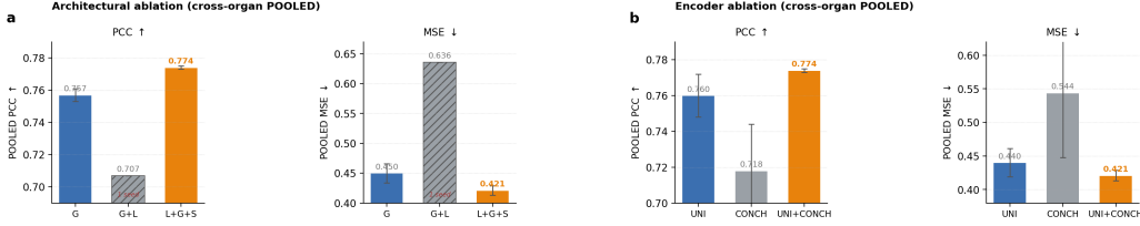
Figure 2: Ablation study on cross-organ POOLED (11-gene leakage-safe panel), each panel reported in both Pearson correlation (PCC \uparrow ) and mean-squared error (MSE \downarrow ). (a) Architectural (context-stream) ablation: global attention only (G), global + local (G+L), and the full model (L+G+S; local + global + slide). The full model is best on both PCC (0.774) and MSE (0.421); the G+L bar is hatched as it currently has a single seed (remaining stream configurations are still training). (b) Feature-encoder ablation: UNI, CONCH, and UNI+CONCH frozen features; UNI+CONCH is best on both PCC (0.774) and MSE (0.421). Orange marks the full model / best encoder; error bars are std over three seeds.
