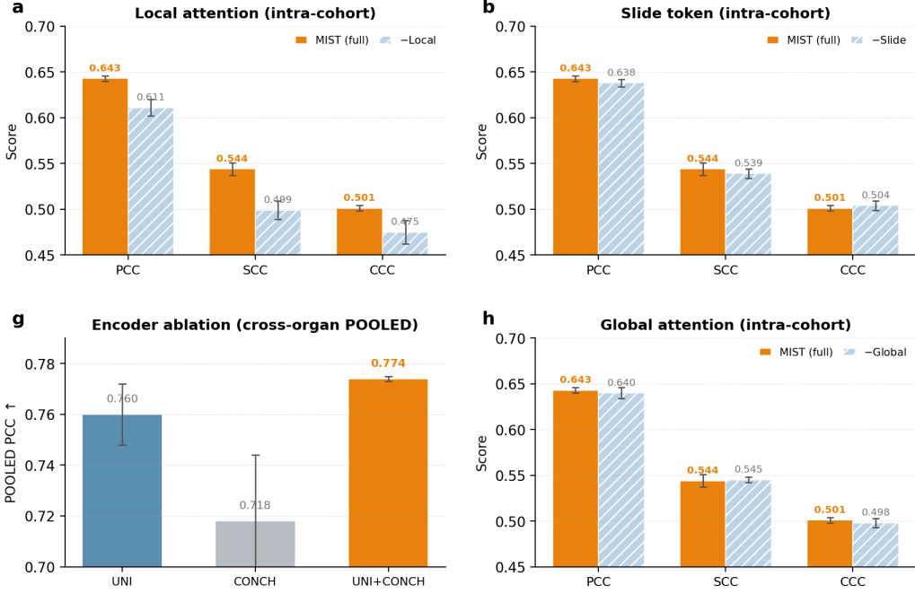
Figure 2: Ablation study. (a,b,h) Architectural stream ablations (intra-cohort, SKCM + LUNG, three seeds): full MIST versus removing the (a) local-attention, (b) slide-token, or (h) global-attention stream, each across Pearson (PCC), Spearman (SCC), and concordance (CCC) correlation. Local attention is the dominant contributor (+0.032 PCC); slide and global add little ( \leq 0.005 PCC), consistent with Table 6. (g) Feature-encoder ablation on cross-organ POOLED (11-gene leakage-safe panel): UNI, CONCH, and UNI + CONCH frozen features; UNI + CONCH is best overall (0.774; +0.014 over UNI, +0.056 over CONCH). Orange marks the full model / best encoder; error bars are std over three seeds.
