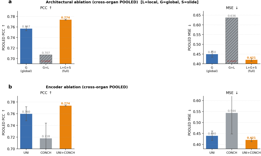
Figure 2: Ablation study on cross-organ POOLED (11-gene leakage-safe panel), each panel reported in both Pearson correlation (PCC \uparrow ) and mean-squared error (MSE \downarrow ). (a) Architectural (context-stream) ablation: global attention only (G), global + local (G+L), and the full model (L+G+S; local + global + slide). The full model is best on both PCC (0.774) and MSE (0.421); the G+L bar is hatched as it currently has a single seed (remaining stream configurations are still training). (b) Feature-encoder ablation: UNI, CONCH, and UNI+CONCH frozen features; UNI+CONCH is best on both PCC (0.774) and MSE (0.421). Orange marks the full model / best encoder; error bars are std over three seeds.
