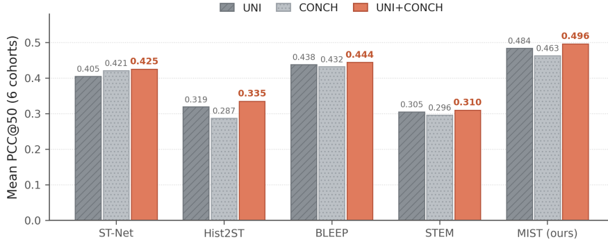
Figure 7: Encoder-averaged intra-cohort PCC@50 per model. Six-cohort mean for each encoder (UNI, CONCH, UNI+CONCH); same values as Table 8. MIST is highest under every encoder, and UNI+CONCH is best for it.
