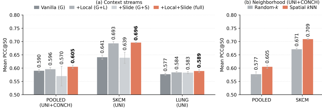
Figure 2: Context-stream ablation: self-attention is the vanilla Transformer backbone; local and slide are the added levers. (a) Context Streams. (b) Neighborhood.
