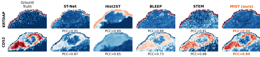
Figure 4: Qualitative spatial expression maps for SKCM slide TENX117 (two marker genes, rows); per-gene PCC shown, MIST in orange. Identical frozen UNI+CONCH features for all methods.
