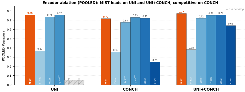
Figure 2: Feature-encoder ablation (cross-organ POOLED, Pearson \uparrow ). Every method is trained identically under the POOLED regime (11-gene leakage-safe panel, three seeds) with three frozen patch encoders—UNI (1024-d), CONCH (512-d), and UNI + CONCH (1536-d). MIST (orange) attains the highest cross-organ transfer under every encoder, and UNI + CONCH is best overall (0.774; +0.014 over UNI, +0.056 over CONCH). Unlike the neighbourhood and context ablations, the encoder choice produces a real, consistent gap—the frozen features are the dominant factor.
