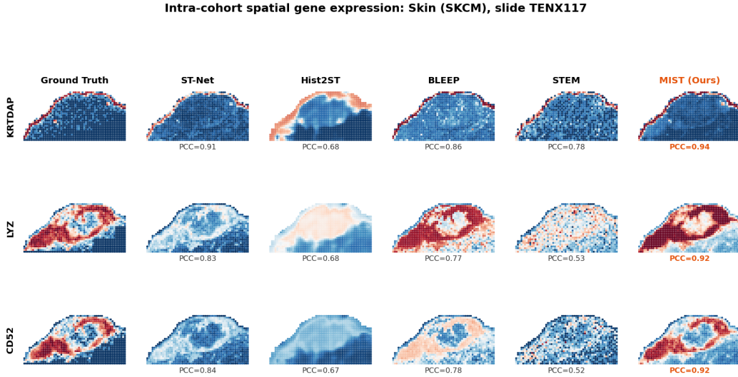
Figure 3: Qualitative spatial expression maps for a held-out skin (SKCM) slide (TENX117), three genes (rows). Each panel colours every spot by expression; MIST (right) most faithfully recovers the ground-truth spatial structure—the perivascular ring for LYZ/CD52 and the epidermal edge for KRTDAP—attaining the highest per-gene PCC (in orange), whereas STEM is noisy and Hist2ST over-smooths. Predictions use identical frozen UNI+CONCH features.
